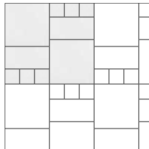
Schema 6 60x60 = 54,55% | 30x60 = 27,27% | 20x20 = 18,18%
