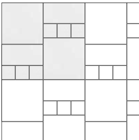
Schema 7 60x60 = 54,55% | 30x60 = 27,27% | 20x20 = 18,18%
