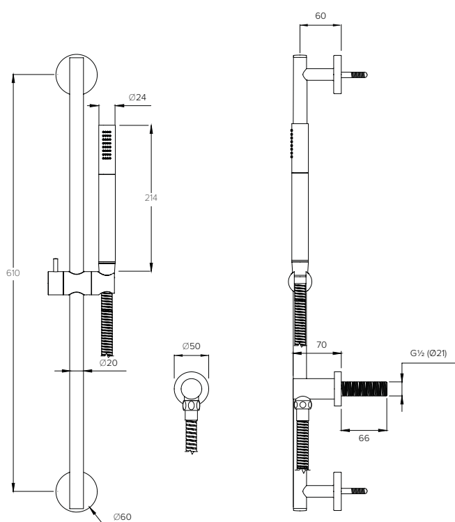
RISER RAIL & PENCIL SHOWER HEAD, OUTLET, HOSE
